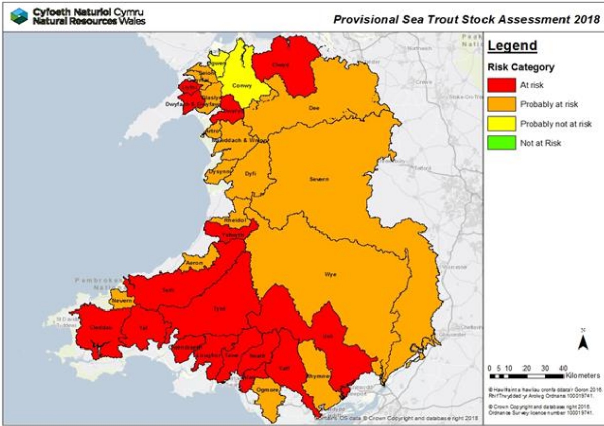
Fig 1 Main sea trout rivers in Wales: Risk status 2018
