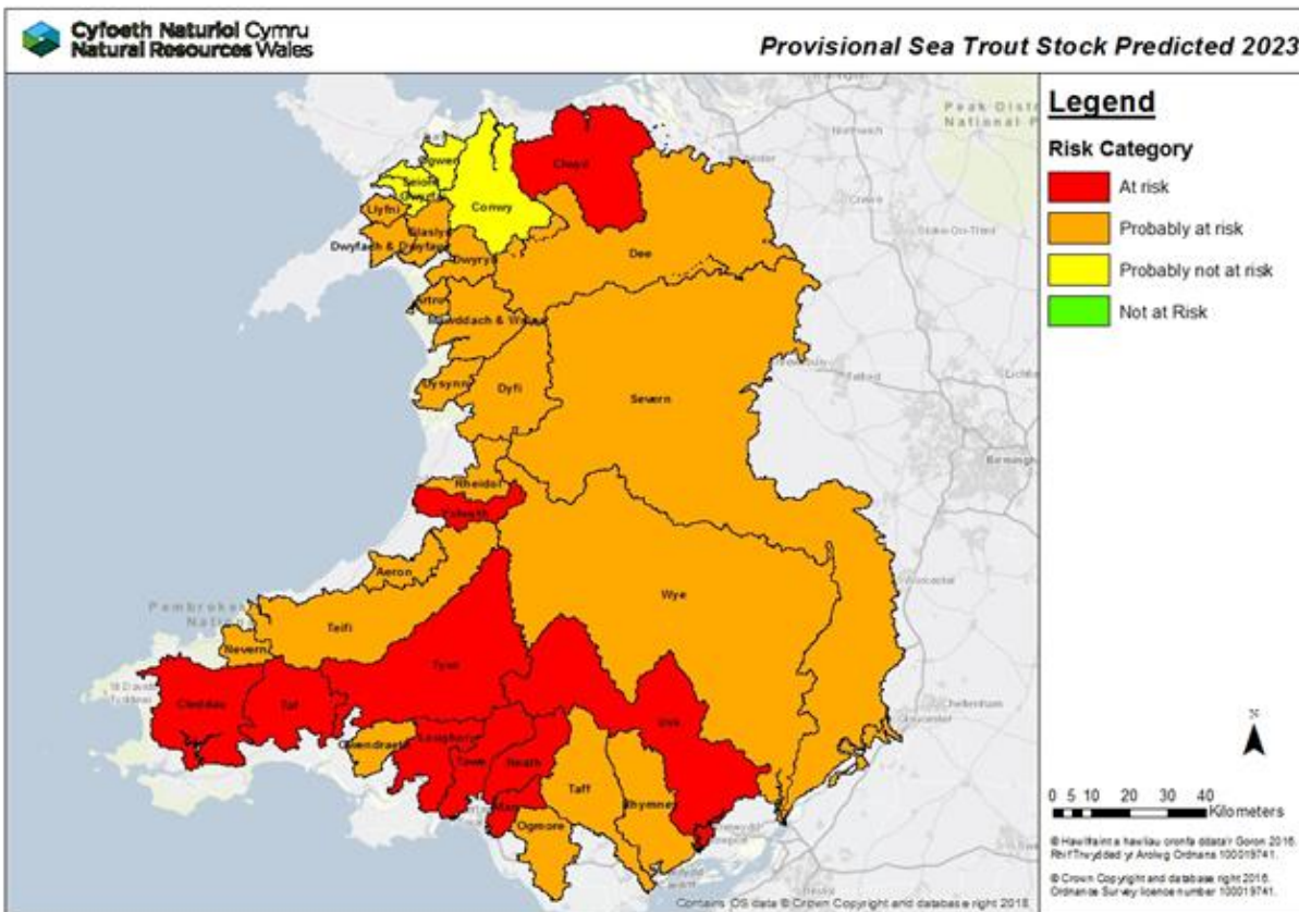
Fig 2 Main sea trout rivers in Wales: Projected risk status 2023
